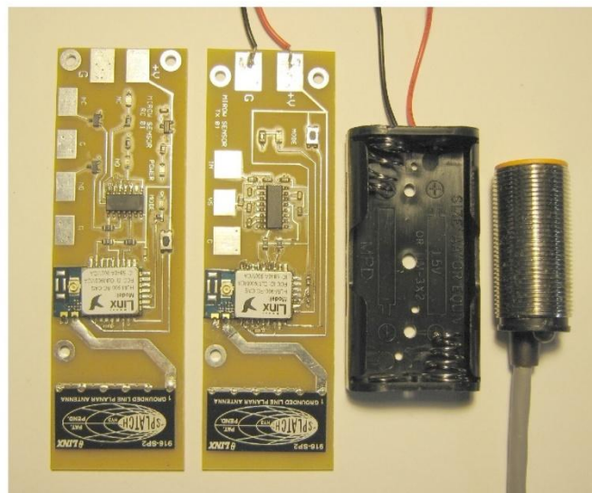
Receiver RC 01 Transmitter TX01 Sensor LPS-M18M3-NO
